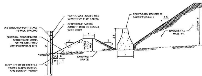
SECTION D - SILT FENCE AND CONTAINMENT BERM NOT TO SCALE
