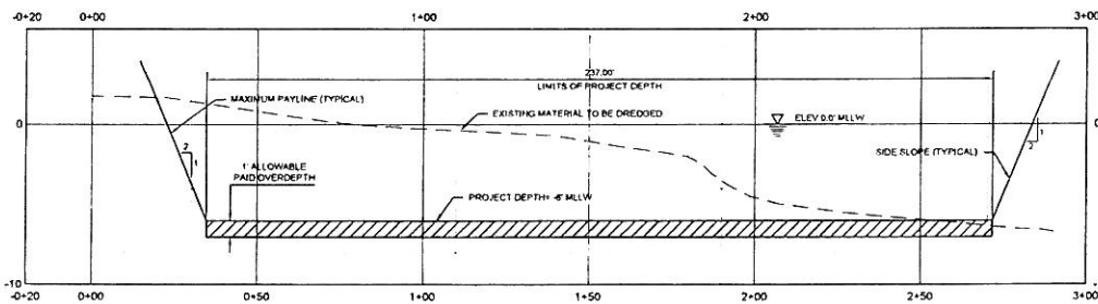
SECTION C
