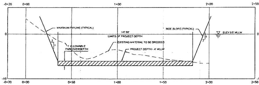
SECTION B
