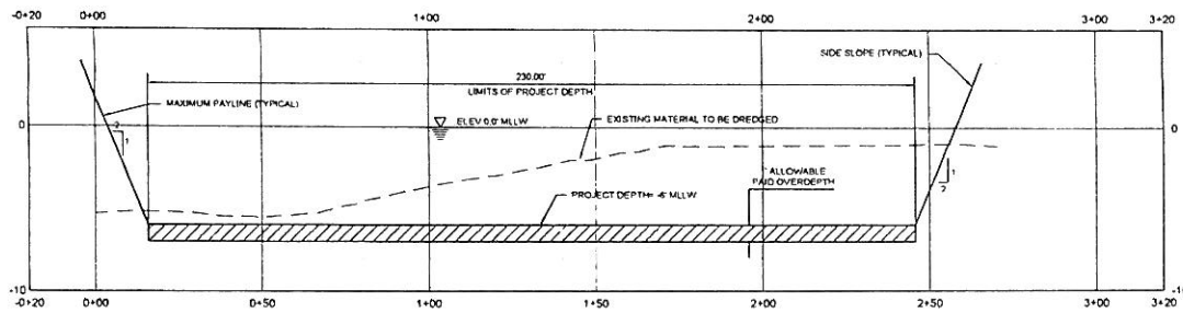
SECTION A
